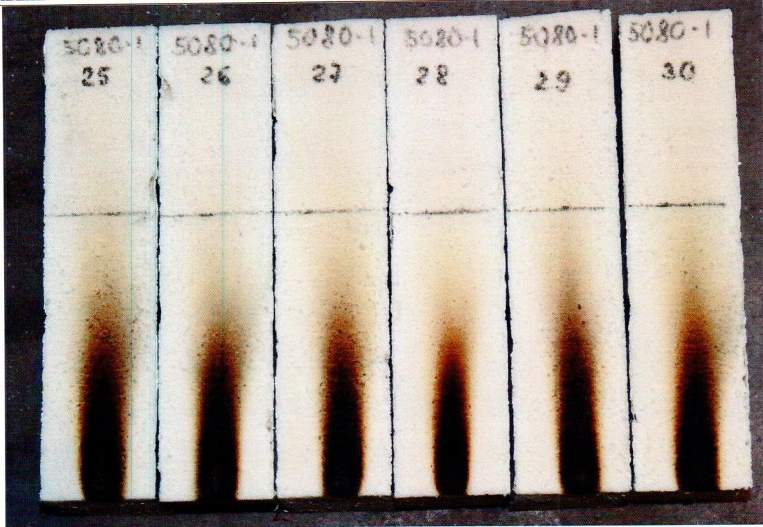
Fig.4. Specimens with 60 mm thickness after tests.
