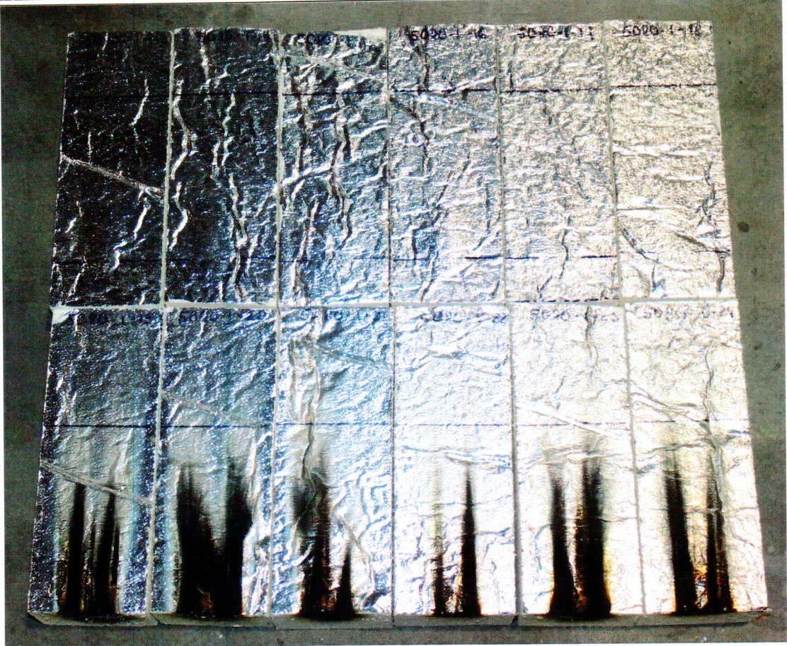
Fig.3. Specimens with 60 mm thickness after tests.
